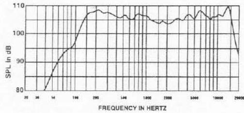
FIGURE 1 — MTH-2.5/64B Axial Frequency Response
